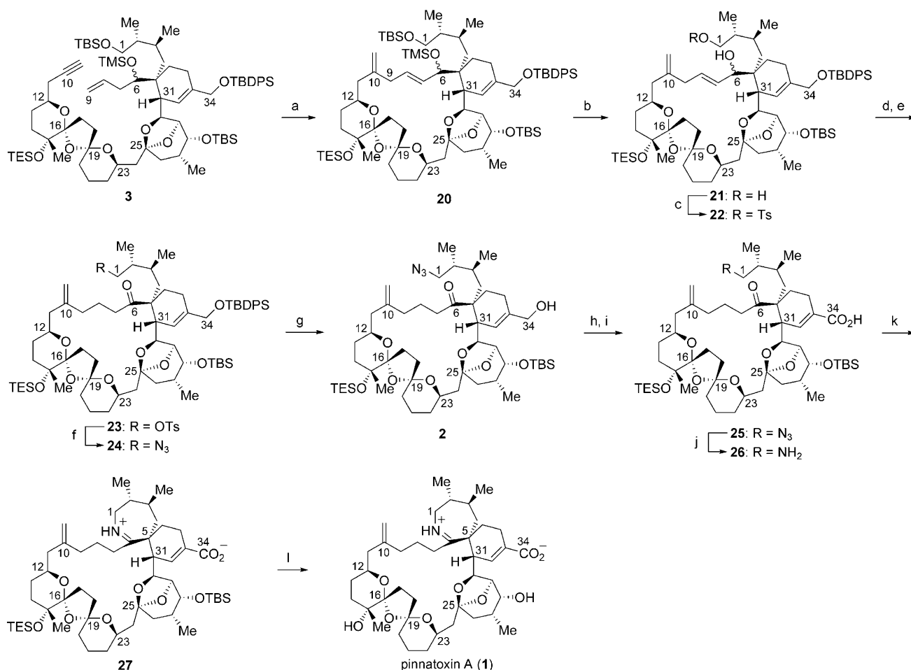
Scheme 3. Completion of the total synthesis of pinnatoxin A ( 1 ). a) [CpRu(MeCN)_3]PF_6 (10 mol %), acetone, 50 °C, 15 min, 79 %; b) PPTS, EtOH, 72 h, 89 %; c) TsCl , pyridine, CH_2Cl_2 , 2 h, 92 %; d) Dess–Martin periodinane, pyridine, CH_2Cl_2 , 6 h; e) [(Ph_3P)CuH]_d , wet benzene, 12 h, 93 % (2 steps); f) NaN_3 , DMF, 70 °C, 18 h, 93 %; g) Bu_4NF , THF, 0 °C, 10 h, 95 %; h) Dess–Martin periodinane, pyridine, CH_2Cl_2 , 1 h; i) NaClO_2 , NaH_2PO_4 , 2-methyl-2-butene, tBuOH/H_2O (4:1), 6 h, 80 % (2 steps); j) H_2 , Lindlar's catalyst, EtOH, 36 h, 83 %; k) chlorobenzene, 120 °C, 18 h, 74 % (84 % based on recovered ketoamino acid 26 ); l) 46 % aqueous HF/MeCN (1:9), 12 h, 91 %. Cp = cyclopentadienyl; Ts = p -toluenesulfonyl.
