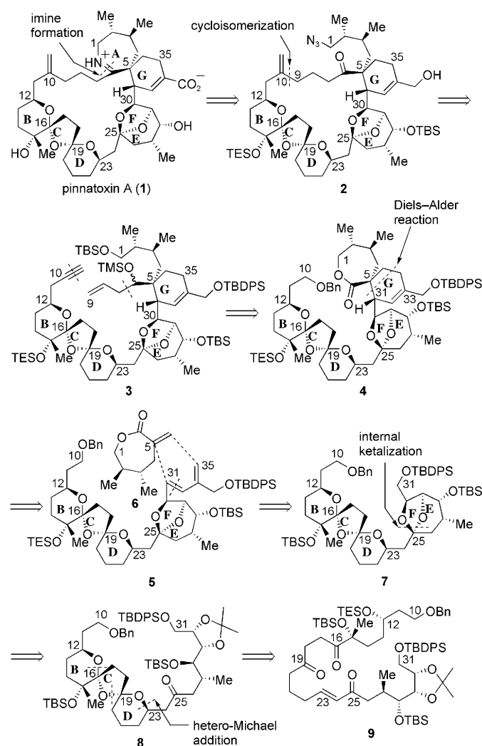
Scheme 1. Retrosynthetic analysis of pinnatoxin A ( 1 ). Bn = benzyl; TBDPS = tert -butyldiphenylsilyl; TBS = tert -butyldimethylsilyl; TES = triethylsilyl; TMS = trimethylsilyl.
